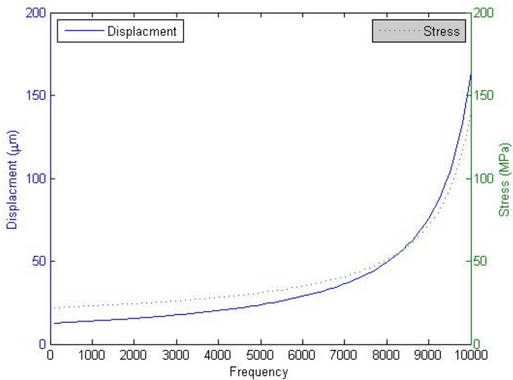
Figure 8 Frequency dependence of displacement and stress
